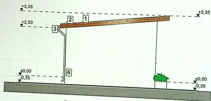
FATADA LATERALA STANGA
